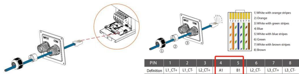
EV Charger COM interface
